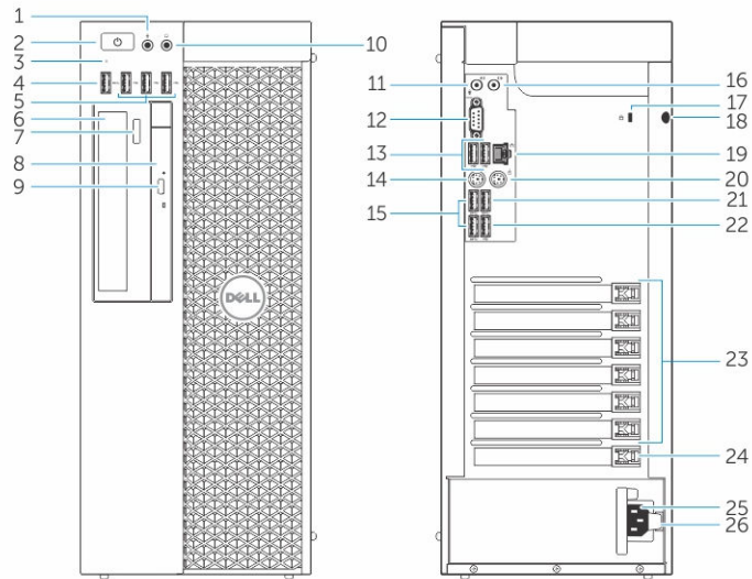
Figure 1. Front and Back View of T7810 Computer
